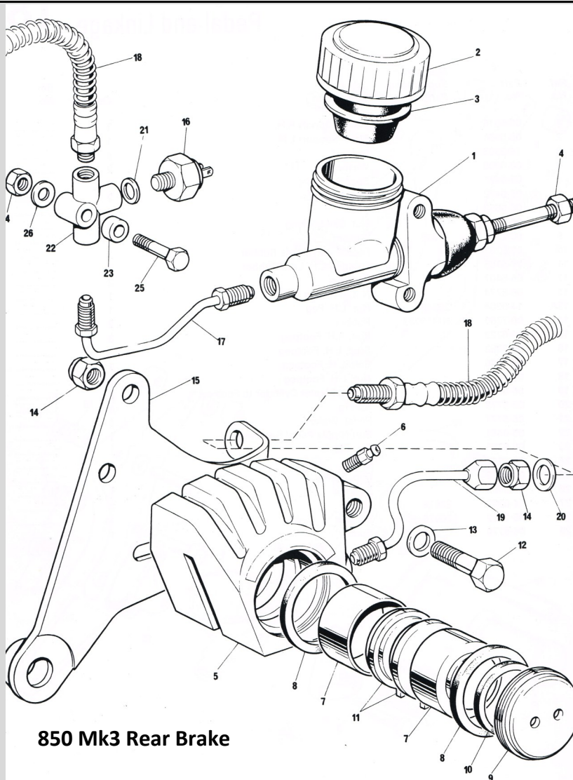
Fluid Reservoir, Master Cylinder
